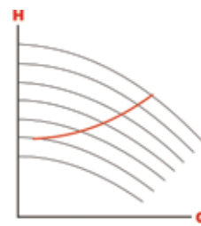
System Curve
