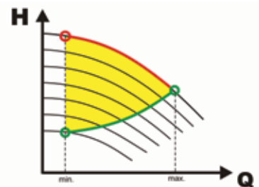
Pressure control, along a system curve (automatic compensation of pipe losses)
