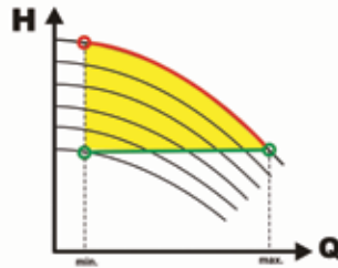
Constant pressure control
