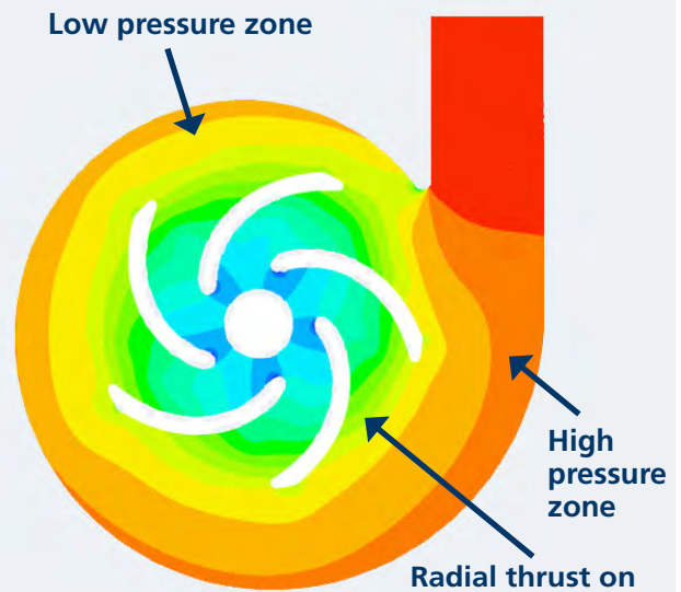
millMAX Standard Volute Design
